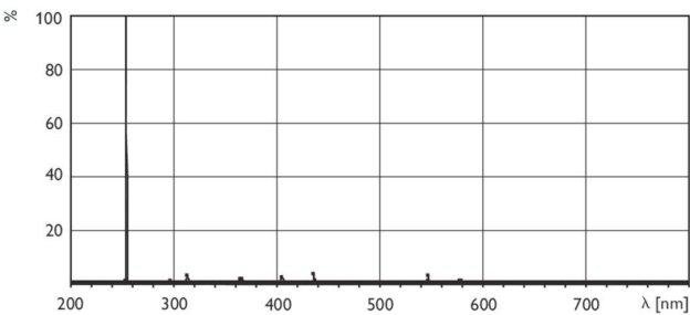
XDPB_XDTUVXPT-Spectral power distribution B/W
